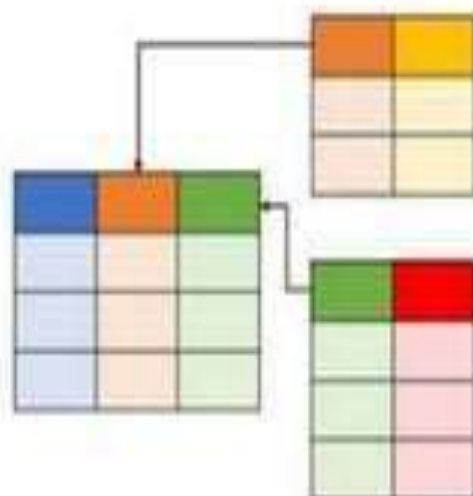
Relational
