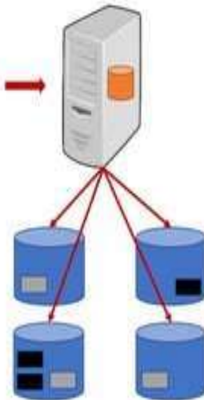
Data storage
