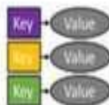
Key-Value
