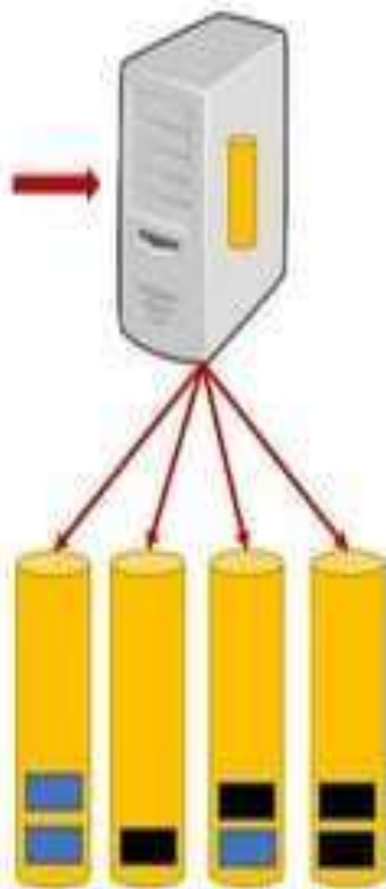
Data Ingestion
