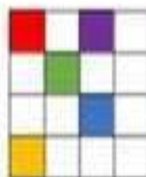
Column
